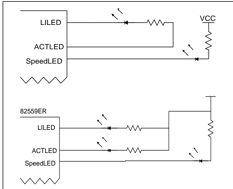
Figure 16. Two and Three LED Schematic Diagram
