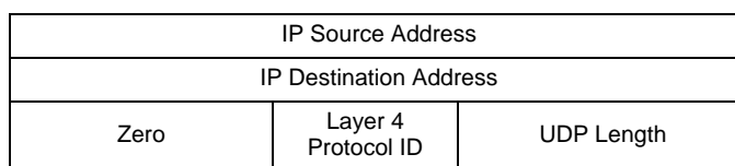
Figure 3-17. UDP Pseudo Header Diagram for IPv4
